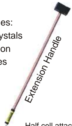
Half cell attached to T&R CP voltmeter. Extension handles also available.
